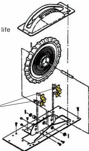
Trim wheel stop catch
